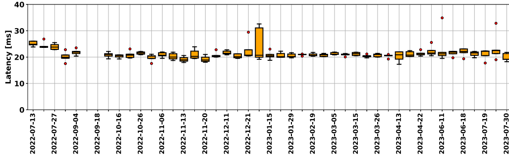
Fig. 17. Single UE latency under static conditions.
