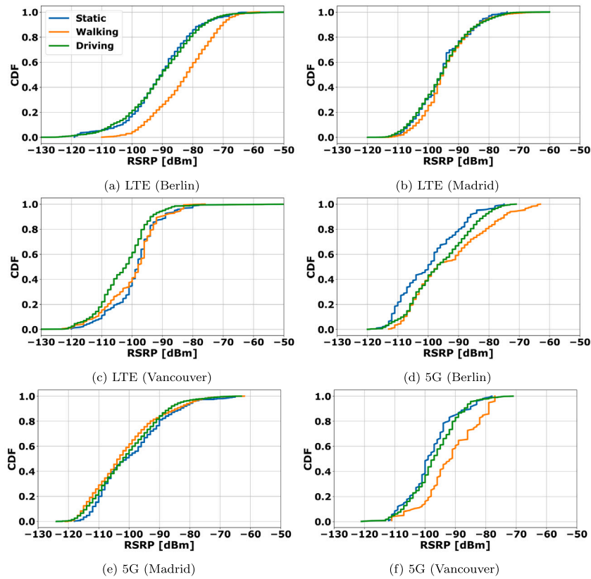
Fig. 10. RSRP comparison across different mobility modes (Static: blue, Walking: orange, Driving: green).
