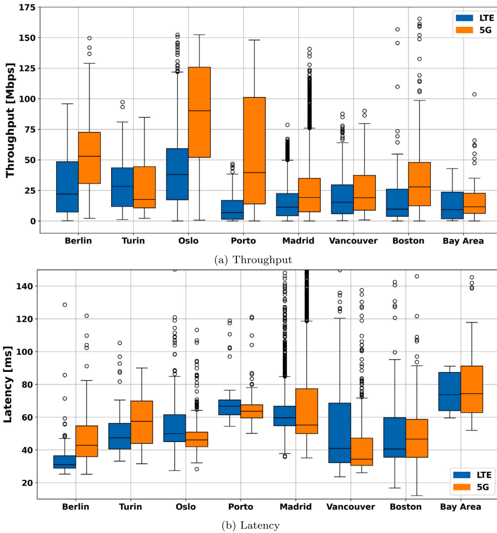
Fig. 11. Technology-wise comparison across different cities (LTE: blue, 5G: orange).
