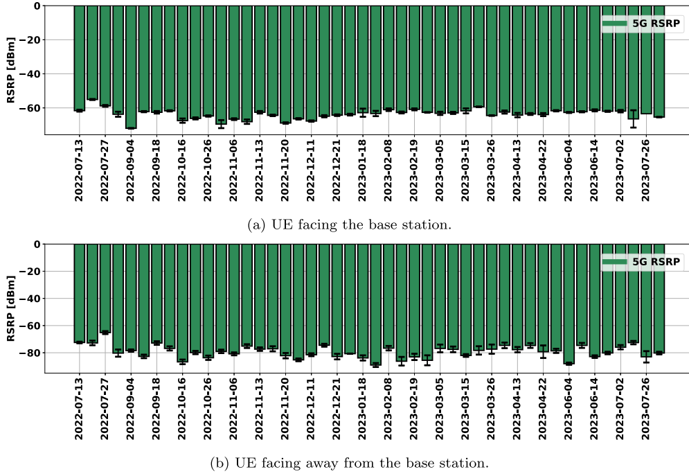
Fig. 14. Single UE daily average RSRP under static conditions.
