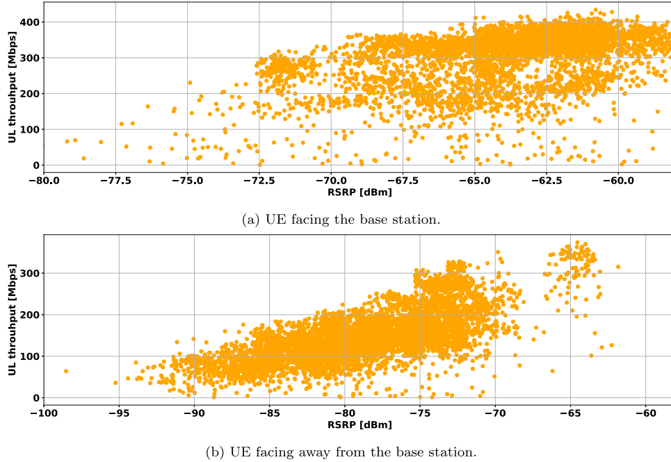
Fig. 15. Single UE throughput vs. RSRP.
