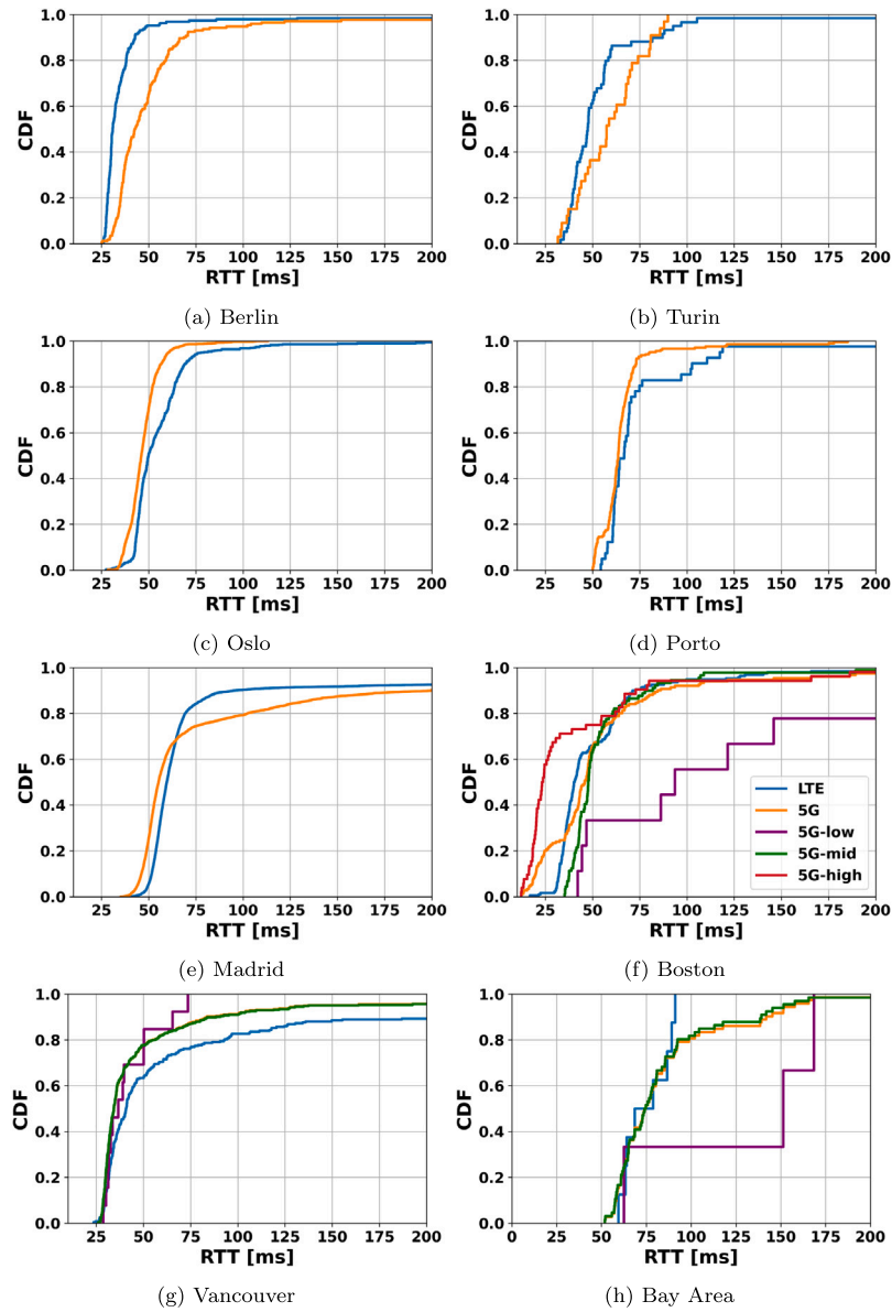
Fig. 6. Latency comparison across different cities. LTE: blue, 5G (5G-low/mid/high combined): orange, 5G-low: purple, 5G-mid: green, 5G-high: red. Not all 5G bands are available in every North American city. For instance, Vancouver lacks mmWave base stations, and T-Mobile in the Bay Area does not offer 5G mmWave service.
