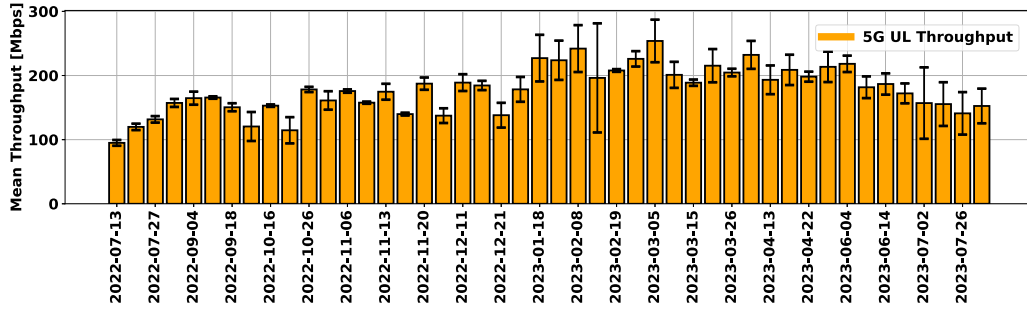
Fig. 18. Single UE throughput during mobility.
