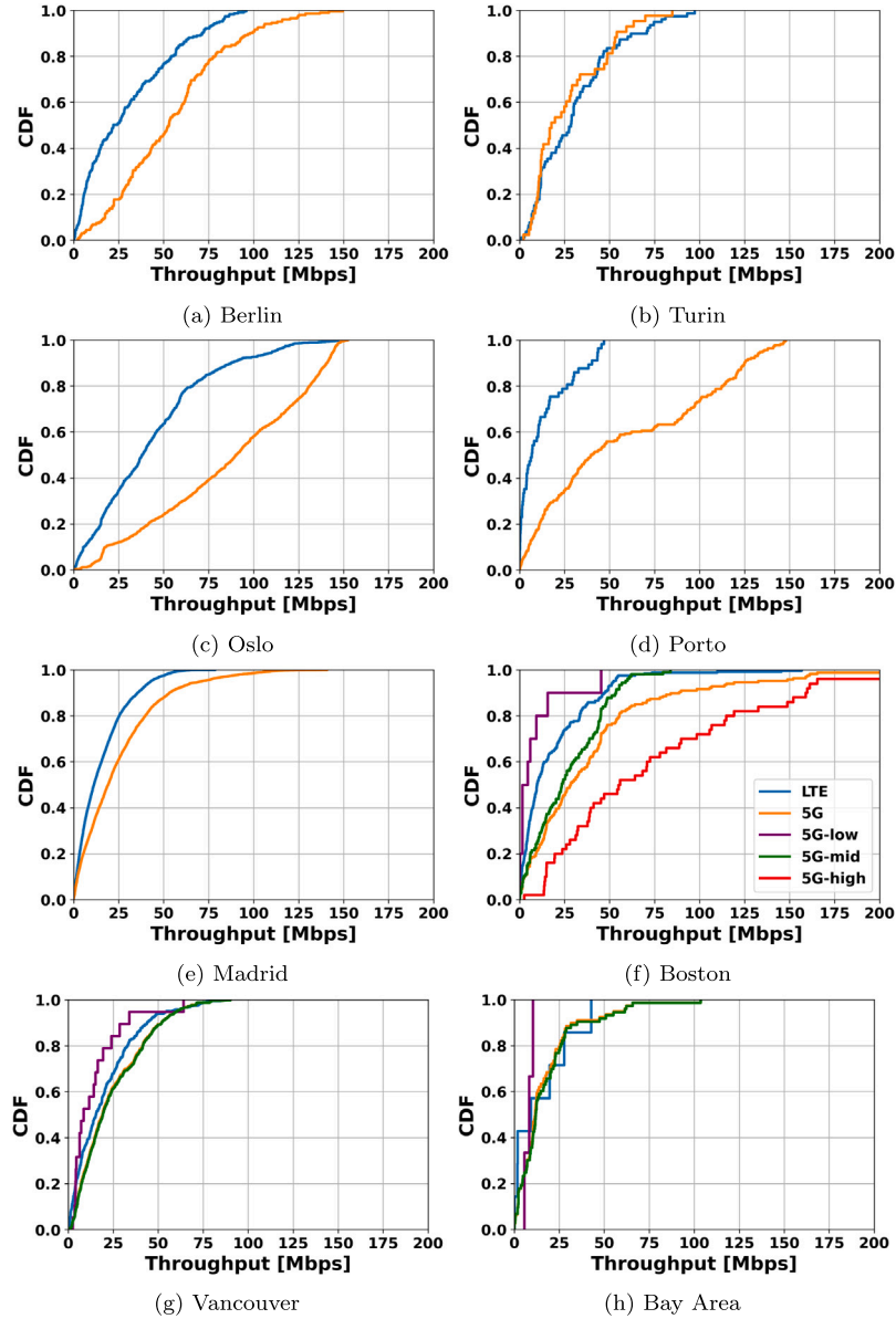
Fig. 5. Throughput comparison across different cities. LTE: blue, 5G (5G-low/mid/high combined): orange, 5G-low: purple, 5G-mid: green, 5G-high: red. Not all 5G bands are available in every North American city. For instance, Vancouver lacks mmWave (5G-high) base stations, and T-Mobile in the Bay Area does not offer 5G mmWave service.
