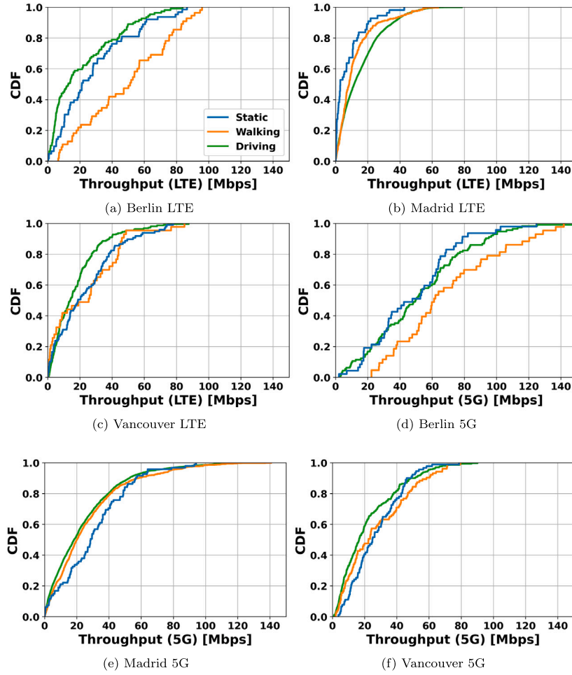
Fig. 8. Throughput Comparison across different mobility modes (Static: blue, Walking: orange, Driving: green).
