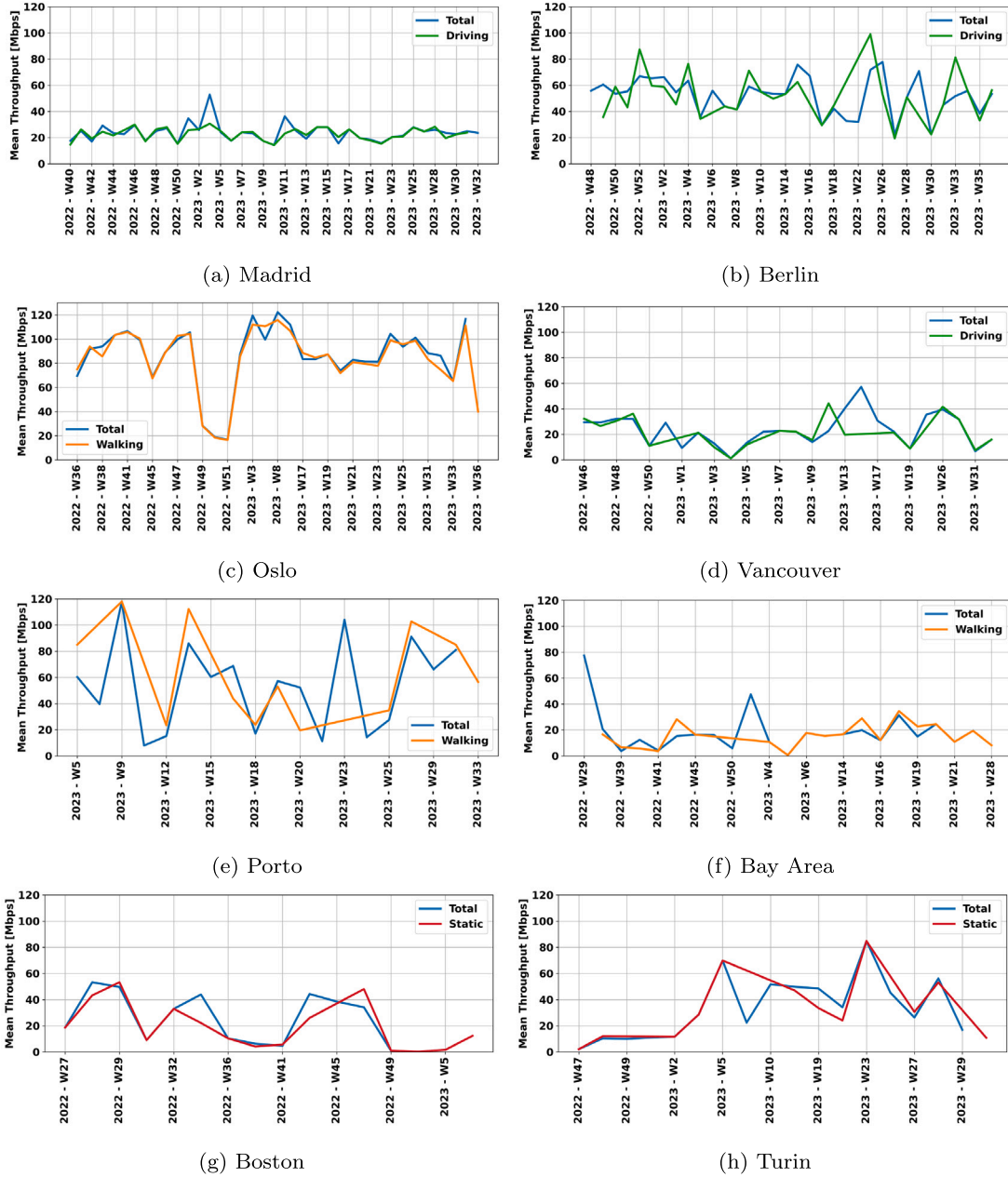
Fig. 3. Evolution of 5G in terms of throughput. Throughput samples collected over a week are averaged and the average throughput over each week is plotted as a timeline. Blue represents the total samples collected by static, walking, and driving measurements combined. Red represents static, orange represents walking, and green represents driving samples only.
