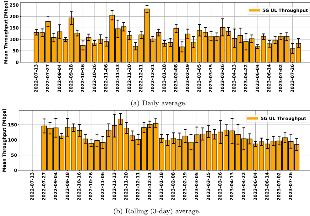
Fig. 13. Single UE static throughput facing away from the base station.
