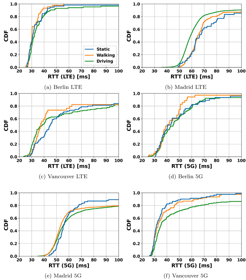
Fig. 9. RTT Comparison across different mobility modes (Static: blue, Walking: orange, Driving: green).
