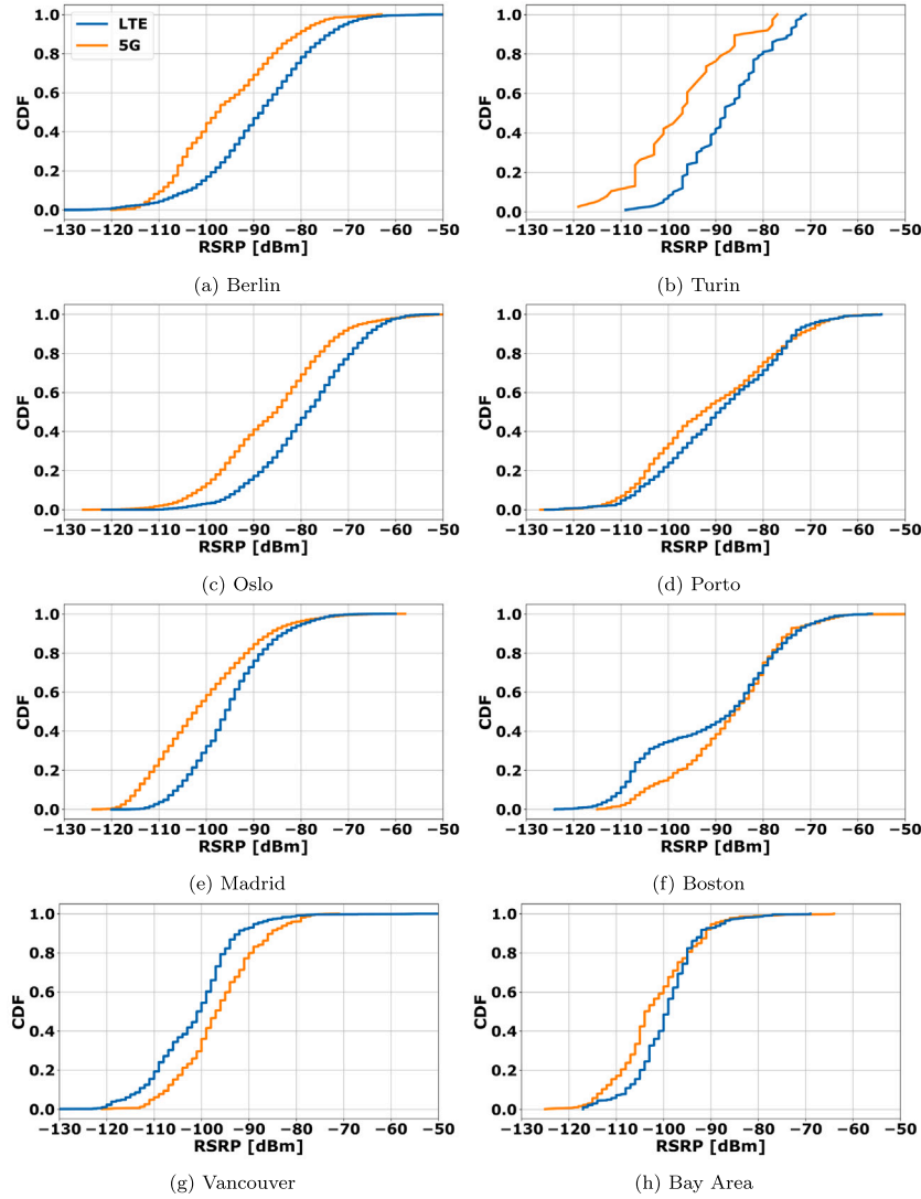
Fig. 7. RSRP comparison across different cities (LTE: blue, 5G: orange).
