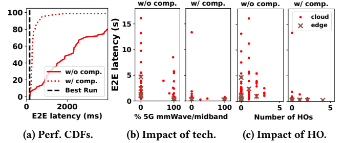
Figure 13: Performance of the AR app with Verizon.
