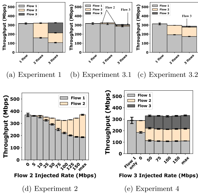
Fig. 12. Replications of experiments 1-4 for uplink.
