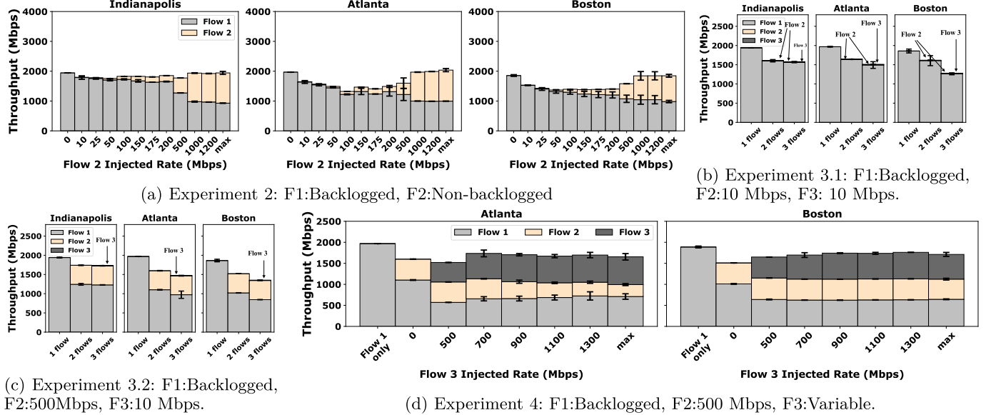
Fig. 7. AT&amp;T, Experiments 2, 3, 4.
