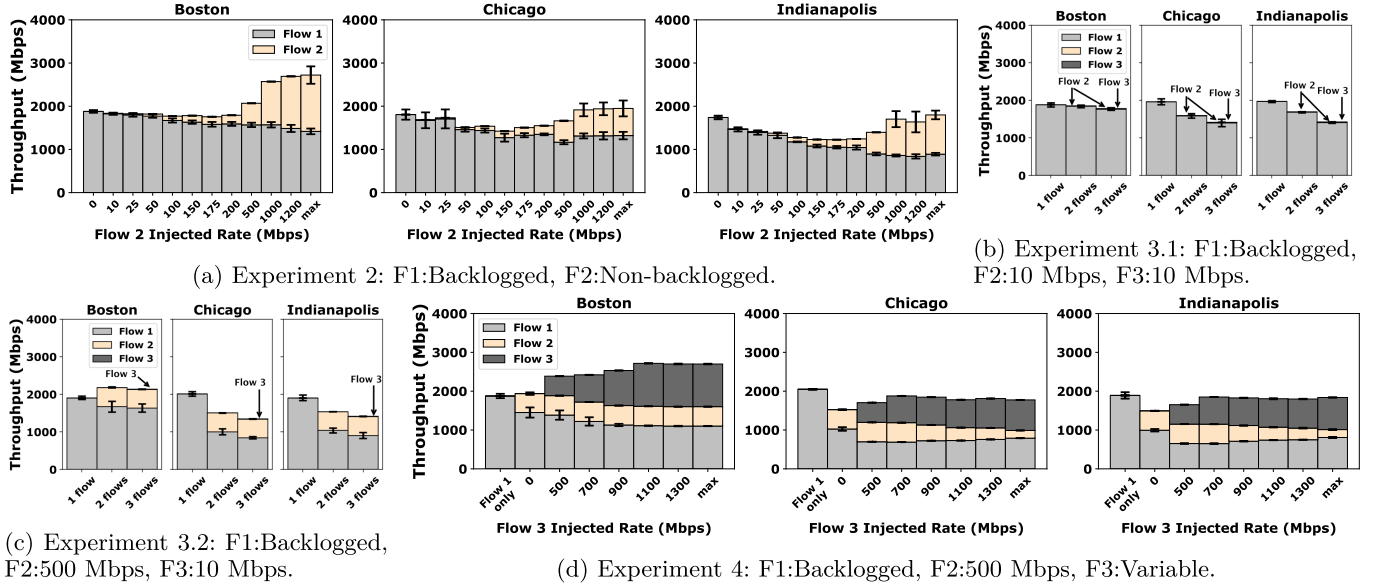
Fig. 6. Verizon, Experiments 2, 3, 4.
