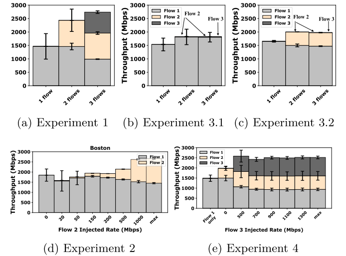
Fig. 16. Verizon: Replications of experiments 1-4 for TCP.
