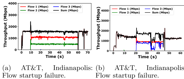
Fig. 19. Measurement timelines for experiment with flow startup failure.
