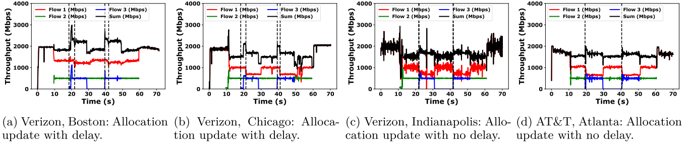
Fig. 17. Measurement timelines for experiments with and without delayed allocation updates.
